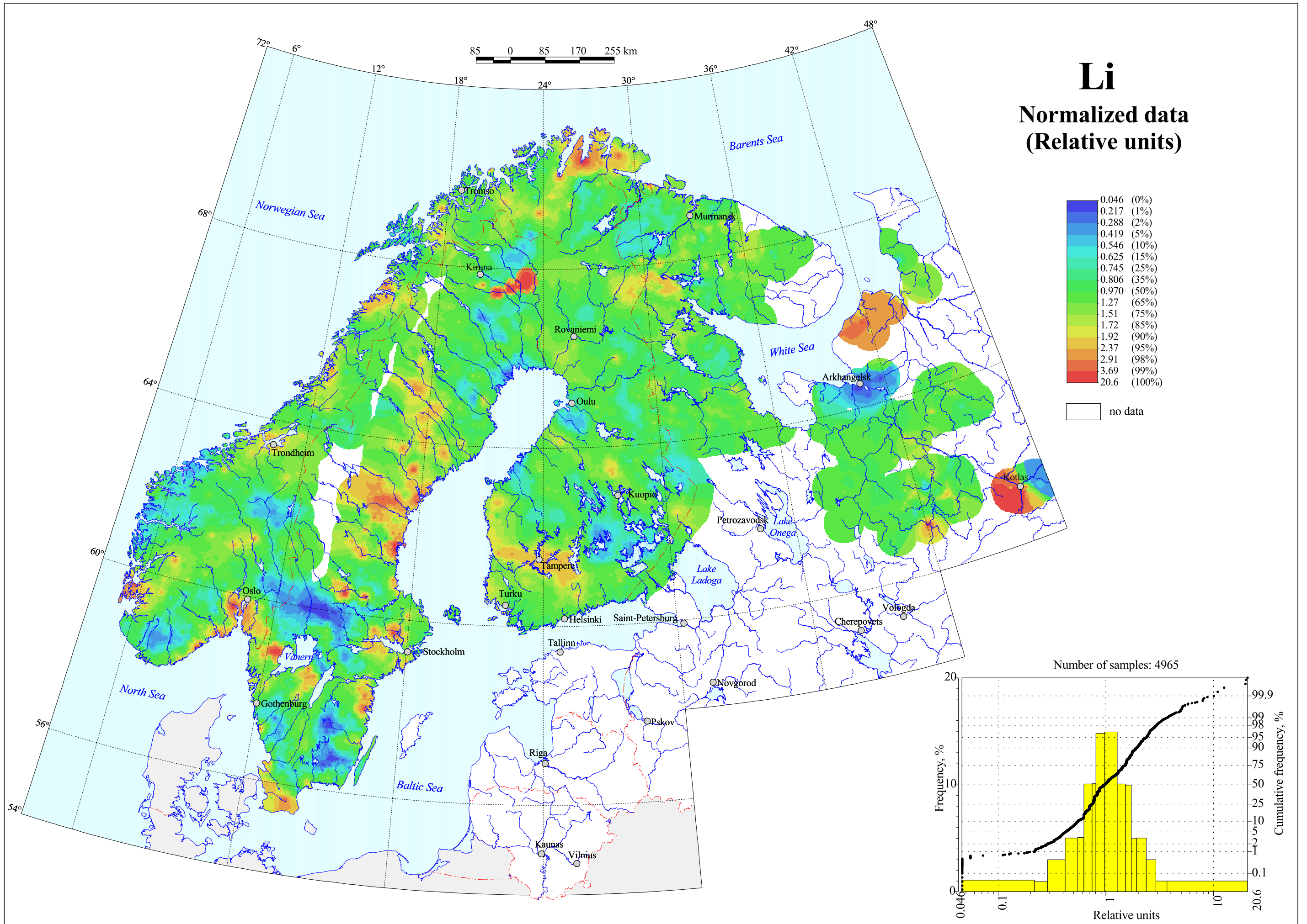
Lithium in Till, Grain Size <0.06 mm
